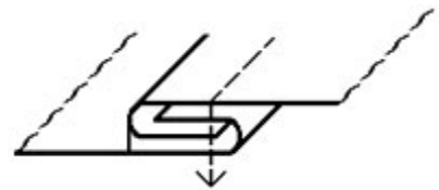
Feet for KHF102 Sleeves Attachment Size between Guide and Needle Hole : 3/16, 1/4, 5/16, 3/8
