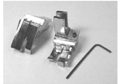
Dual Compensating Feet Enable to obtain Two Different Stitching Margins without changing Presser Foot Adjustable to 1/16 & 1/4 Adjustable to 1/16 & 5/16
